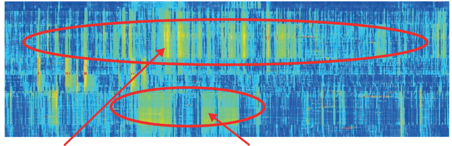
Signal indicating flow through cement channels above SC shoe
