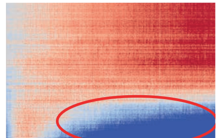
Cooling effect above PC plugs due to gas leak entry point expanding as it passes through plug leak path
